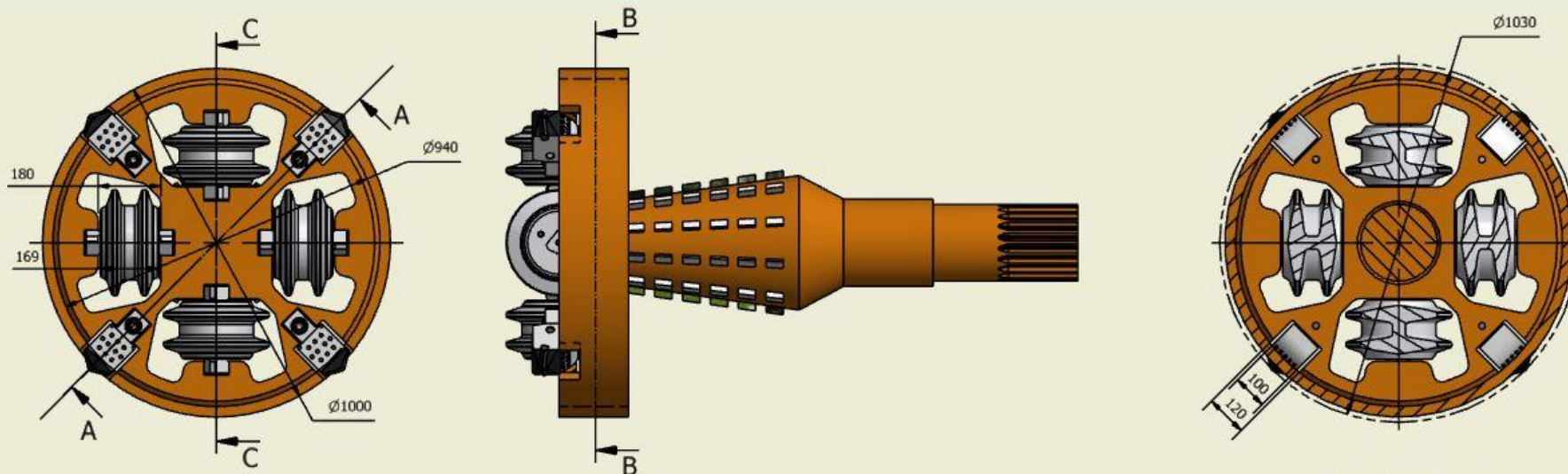
SECTION B-B
